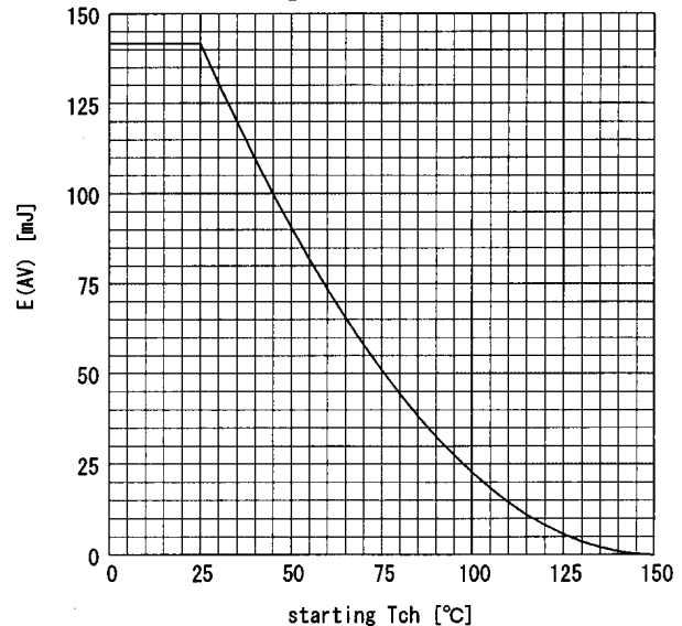
Maximum Avalanche Energy vs. starting T_{ch} E(AV) = f(\text{starting } T_{ch}) : V_{CC} = -24V, I(AV) \geq -7A
